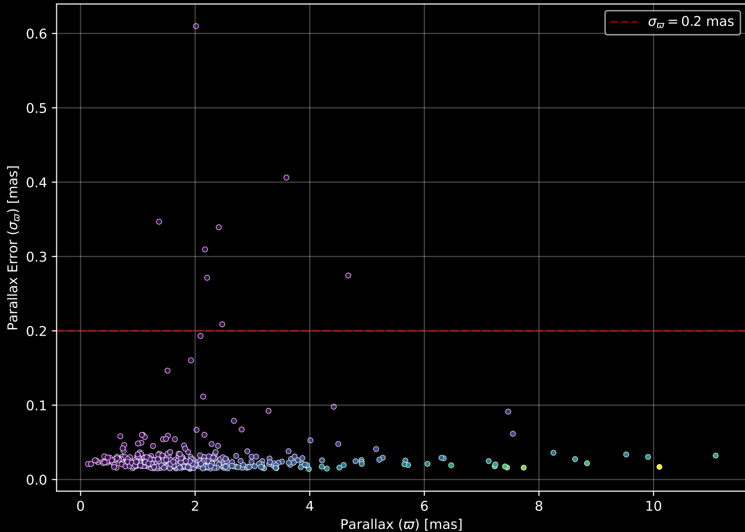
GALAH DR4 Field: [6679] Parallax Quality (n= 408)
