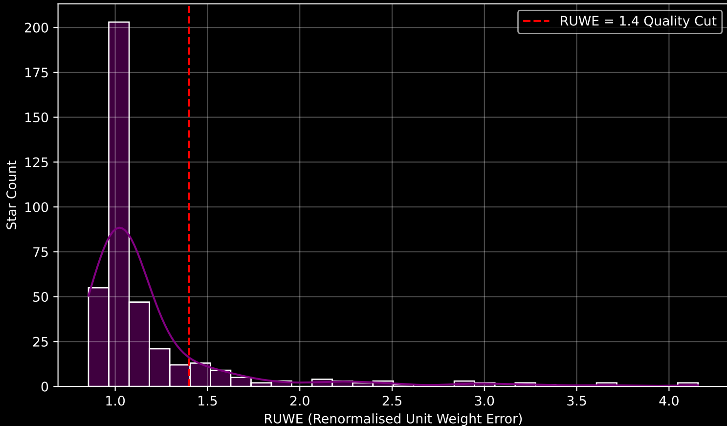
GALAH DR4 Field [6679] RUWE Distribution (n= 395)
