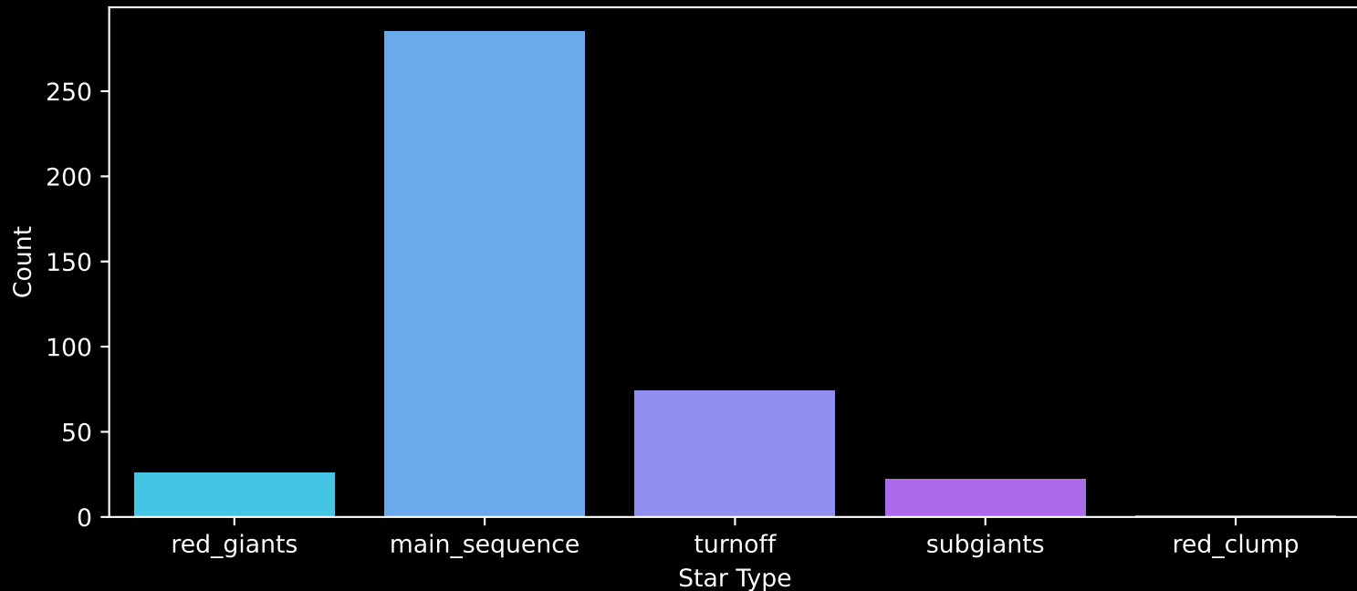
GALAH DR4 Field: [6679] Count plot of Star Type
