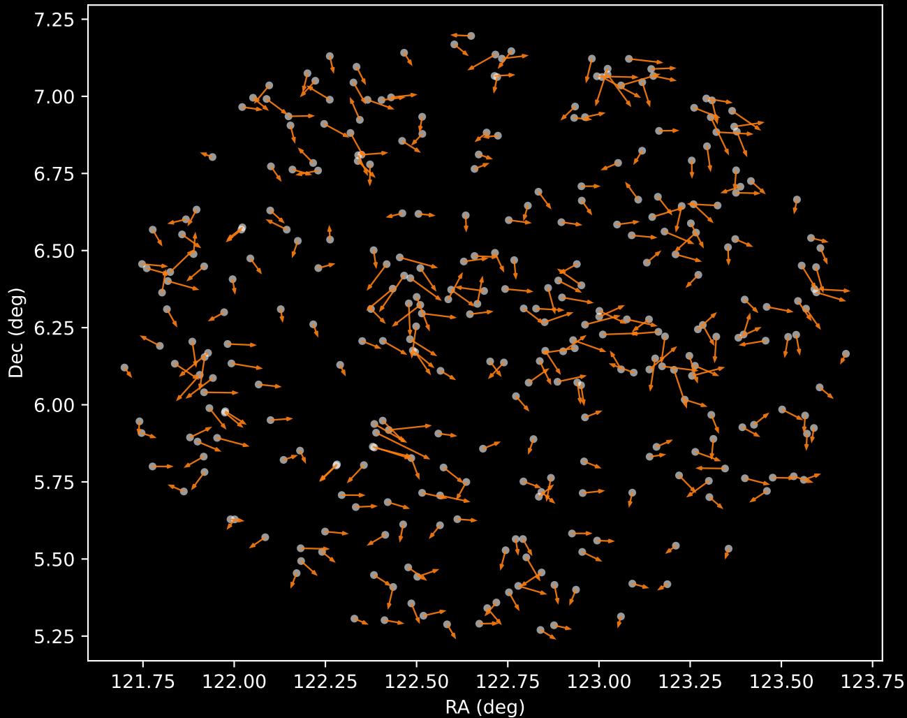
GALAH DR4 Cluster 2 Proper Motion Vectors (n=328)
