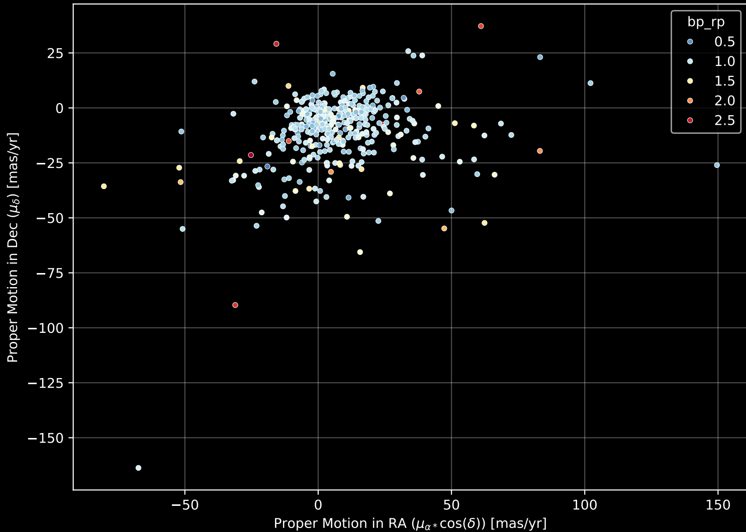
GALAH DR4 Field: [6679] Proper Motion Diagram (n= 408)
